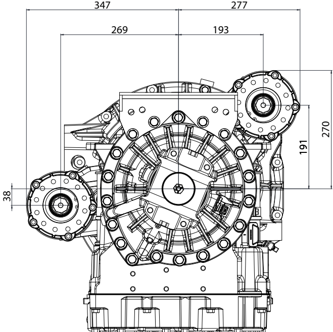
• 83 T - 3000-3200-3500-3700 Side/top
